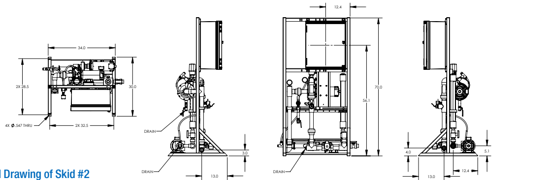
Dimensional Drawing of Skid #2
