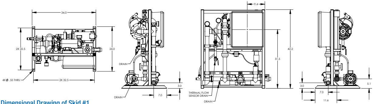
Dimensional Drawing of Skid #1
