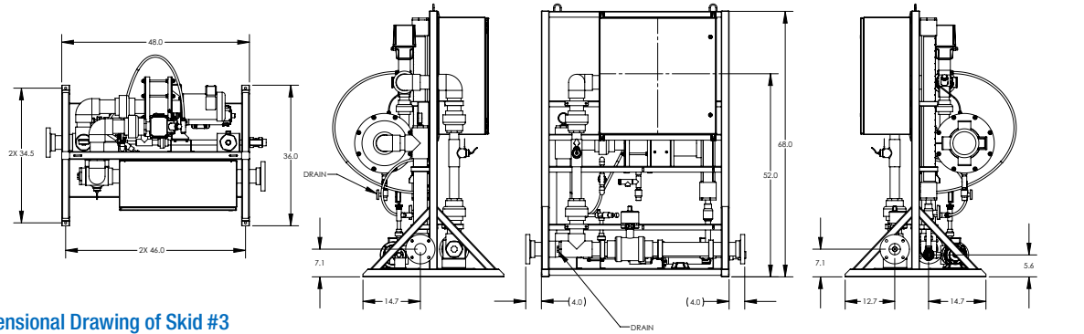
Dimensional Drawing of Skid #3
