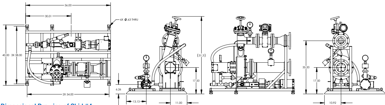
Dimensional Drawing of Skid #4
